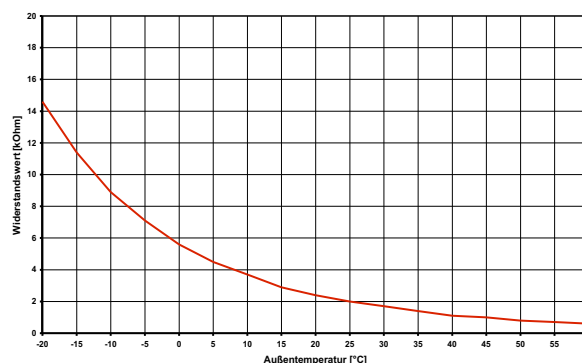
Fig. 8.2: Sensor characteristic curve NTC-2 according to DIN 44574
