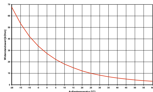
Fig. 9.1: Sensor characteristic curve NTC-10
